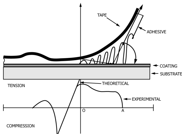
FIG. X1.1 Peel Profile (6)
